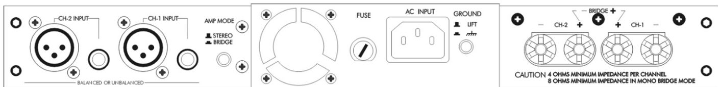
REAR PANELFIGURE
